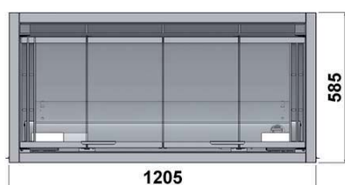
Burner and body assembly - 50 Kg (weight is not inclusive of door assembly shown)
